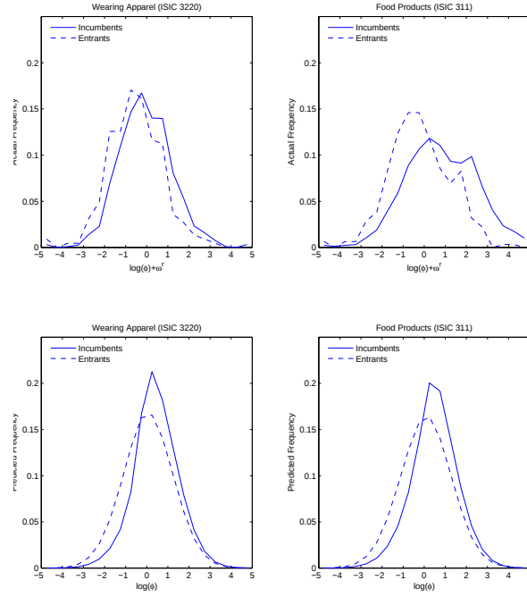
Figure 2: Productivity Distribution of Incumbents and New Entrants (Actual vs. Predicted)
