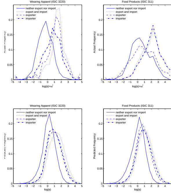
Figure 3: Productivity Distribution across Import/Export Status (Actual vs. Predicted)
